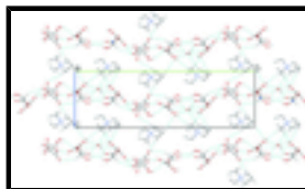
Fig. 3. A view along the a axis of the crystal packing of the title compound, showing both the O—H...O hydrogen bonds and the C—H...O interactions as dashed cyan lines (see Table 1 for details; C-bound H-atoms not involved in the C—H...O interactions have been omitted for clarity).
