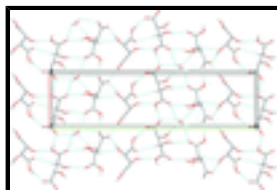
Fig. 2. A view along the c axis of the crystal packing of the title compound, with the O—H...O hydrogen bonds shown as dashed cyan lines (see Table 1 for details; C-bound H-atoms and the Tetra-ethylammonium cations have been omitted for clarity).
